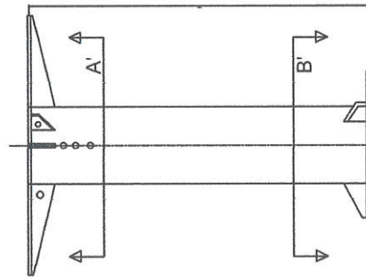
Lantern Support
