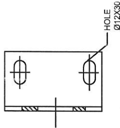
UNION CLAMPS TYPE B UNION B-A-B1
