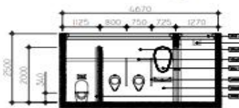
7 SECTION THRU "1-Y" A-2 SCALE 1:100M
