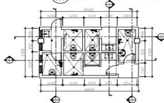
4 SECOND FLOOR PLAN A-I SCALE 1:100H
