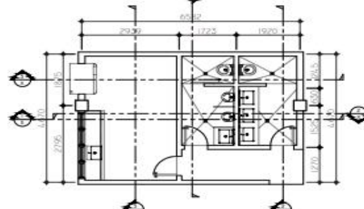
4 THIRD FLOOR PLAN A-2 SCALE 1:100M
