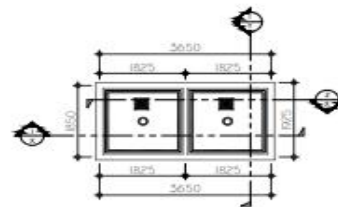
3 REFLECTED CEILING LAYOUT SCALE: 1:100
