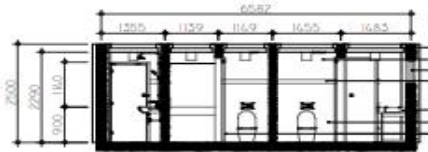
1 SECTION THRU "I-X" A-I SCALE 1:100H
