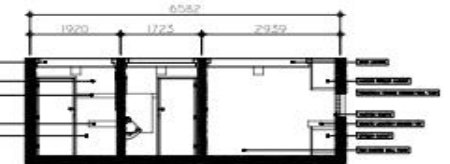
2 SECTION THRU "2-X" A-2 SCALE 1:100M
