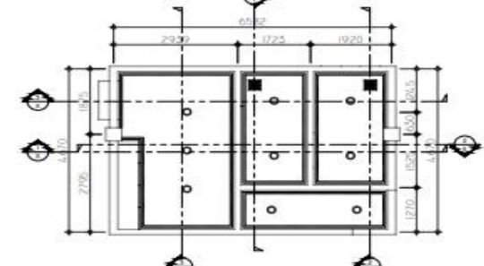
5 REFLECTED CEILING LAYOUT A-2 SCALE 1:100M
