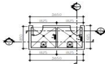
2 GROUND FLOOR PLAN SCALE: 1:100
