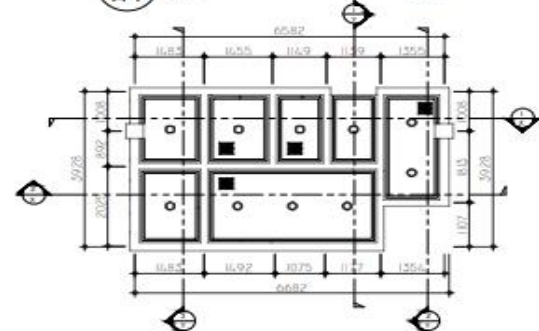
5 REFLECTED CEILING LAYOUT A-I SCALE 1:100H
