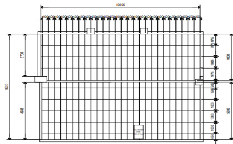
MEZZANINE STEEL FRAME PLAN SCALE 1:1000 MM
